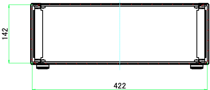
A-A (1:5.5)
